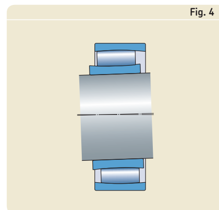
Misaligned and displaced bearing rings
